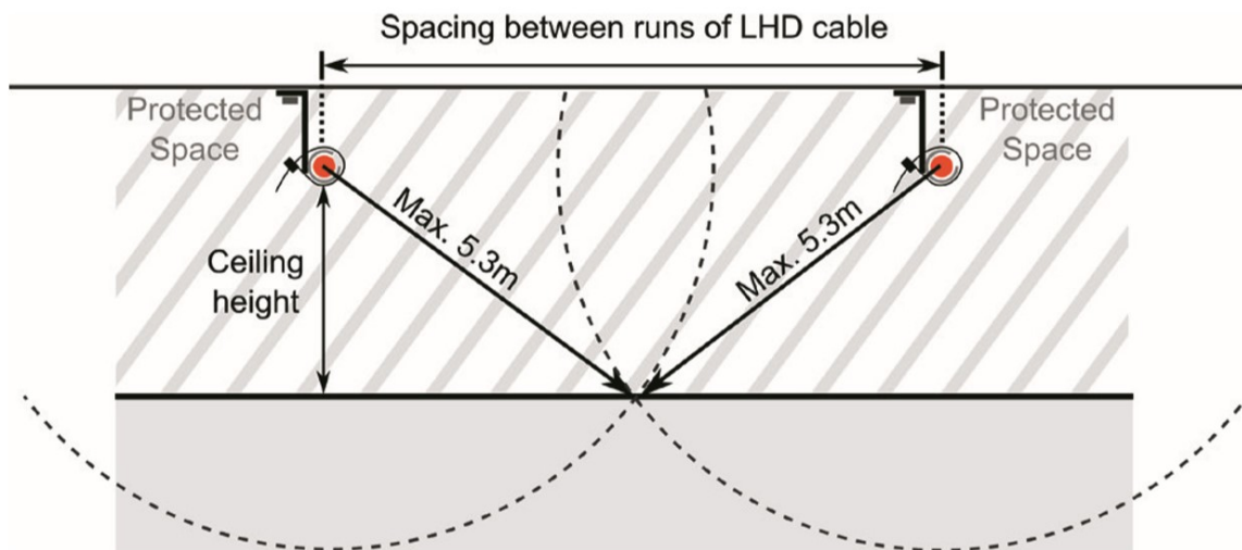
Fig. 5 Spacing requirements for Signaline FT-EN linear heat detection cables
