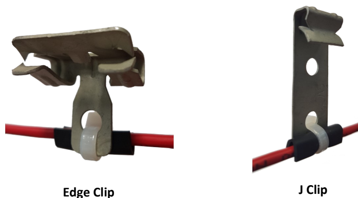
Fig 3. example fixing methods
